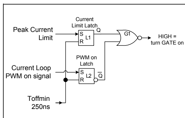
Figure 13 PWM Logic
